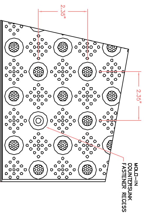
DETAIL 1 ADA PATTERN & FASTENER RECESS
