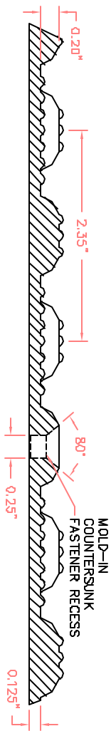
DETAIL 2 LONGITUDINAL CROSS SECTION
